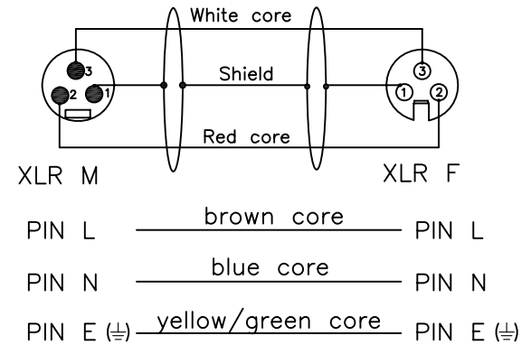
IEC M IEC F Wiring Method(Front View)
