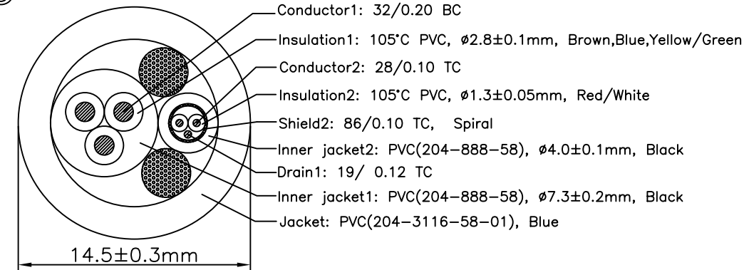
Cable Construction
